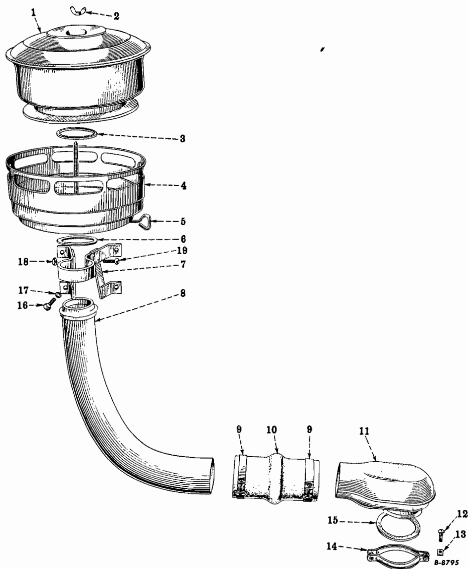
FIG. 12-30 — CARBURETOR AIR CLEANER (Standard) (For SD-240 Gasoline Engines With Carter Carburetor) (For RC-160 Series)
