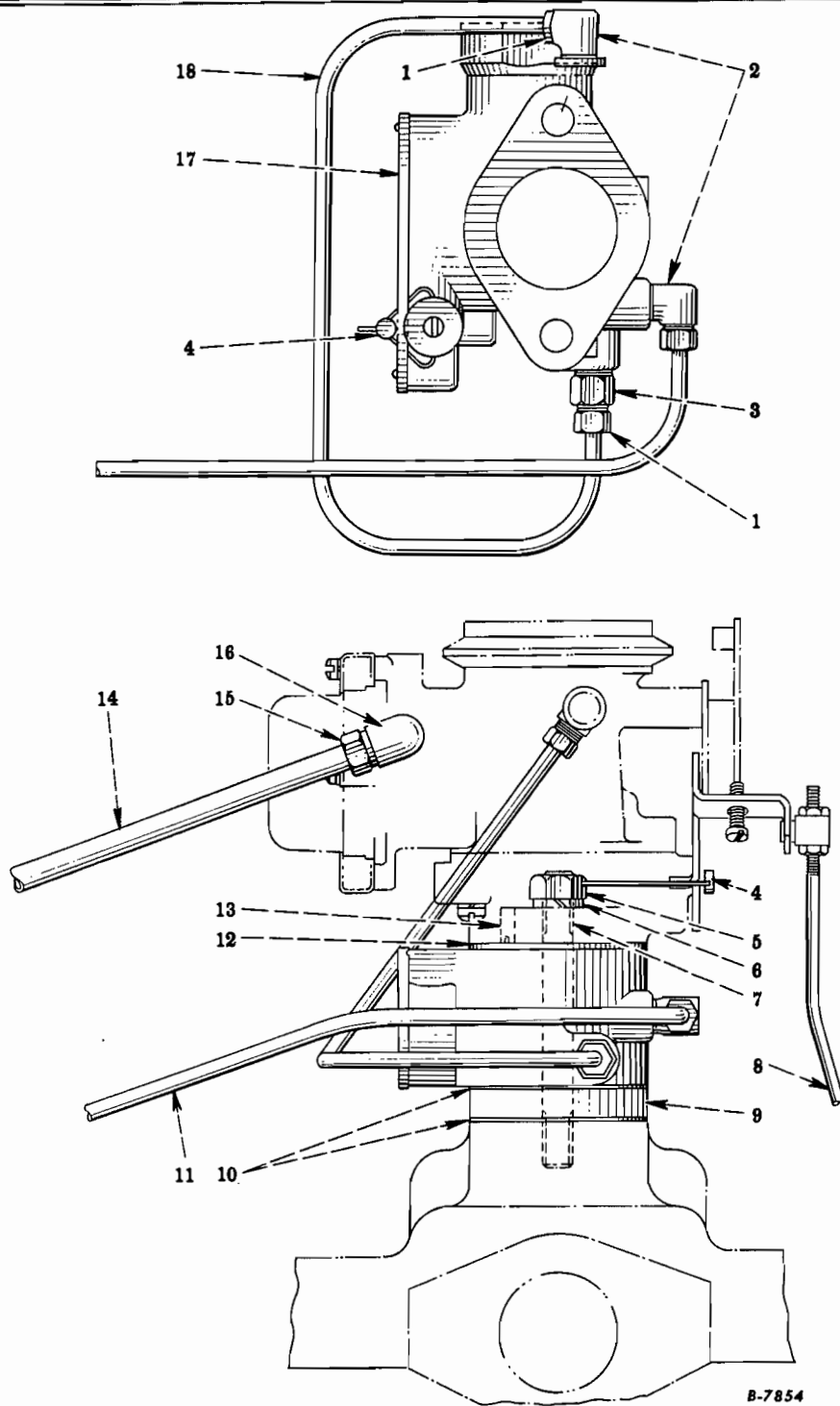
FIG. 12-19 - GOVERNOR AND CARBURETOR MOUNTING (Hoof Governor, Code 1554) (For SD-220 Gasoline Engines, Codes 1201, 1221 and SD-240 Gasoline Engines, Codes 1202, 1212) (R-100 Series - 501 - UP) (R-140 - 4x4 - 501 - UP) (R-110 Series - 8012 - UP) (R-150 Series - 502 - UP) (R-120 Series - 1453 - UP) (R-160 Series - 2986 - UP) (R-130 Series - 1205 - UP) (R-160 - 4x4 - 501 - UP) (RC-160 Series - 761 - UP)
