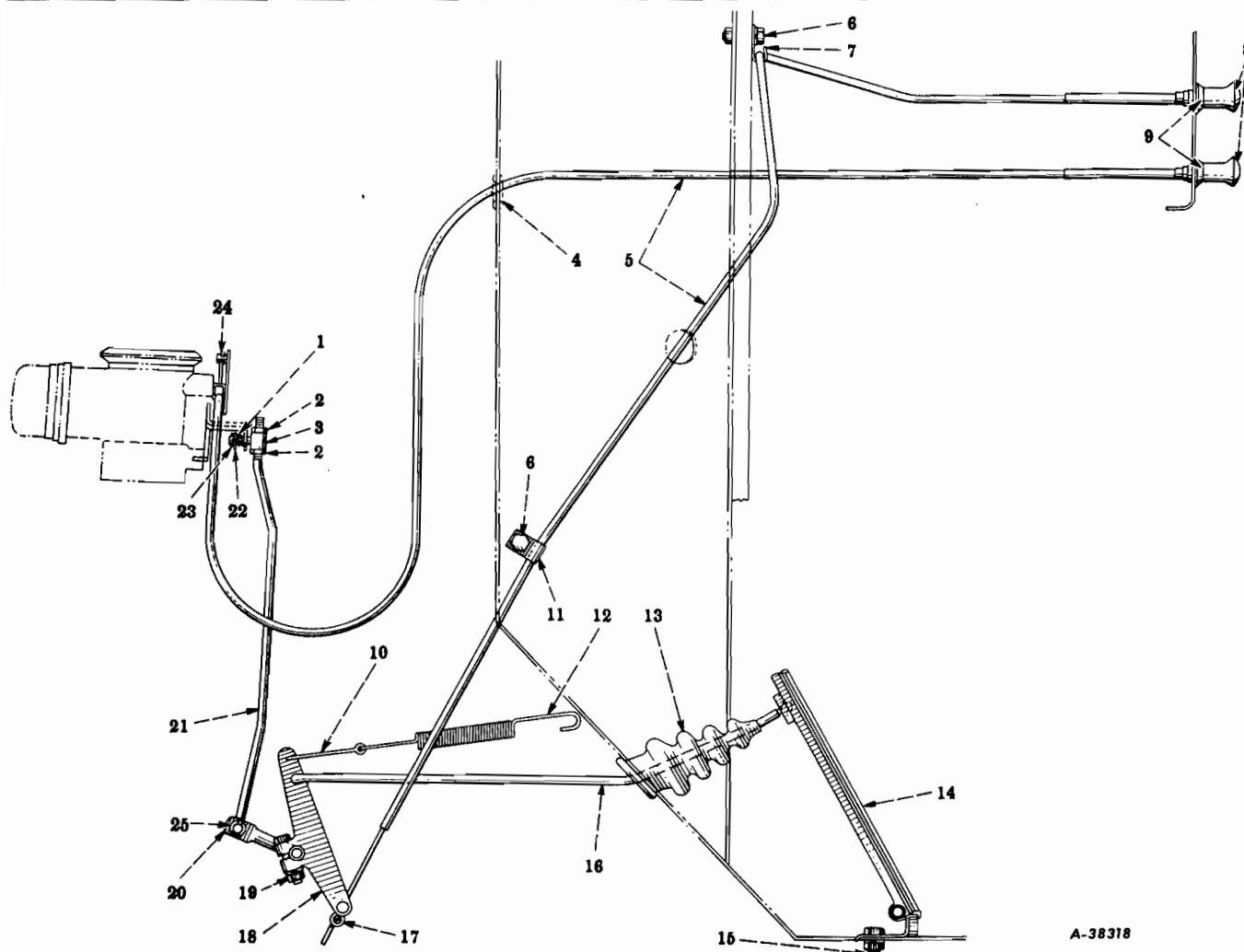
FIG. 12-34 - ACCELERATOR, THROTTLE AND CHOKE CONTROL (Left Hand Drive) (Not For Transmission Code 1374) (All Series Except RC-160)
