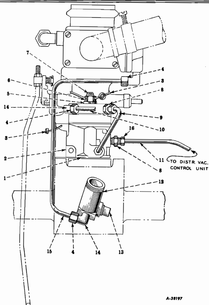
FIG. 12-25 — GOVERNOR AND CARBURETOR MOUNTING (Hoof Governor, Code 1554) (For SD-240 LPG Engines, Code 1231)
