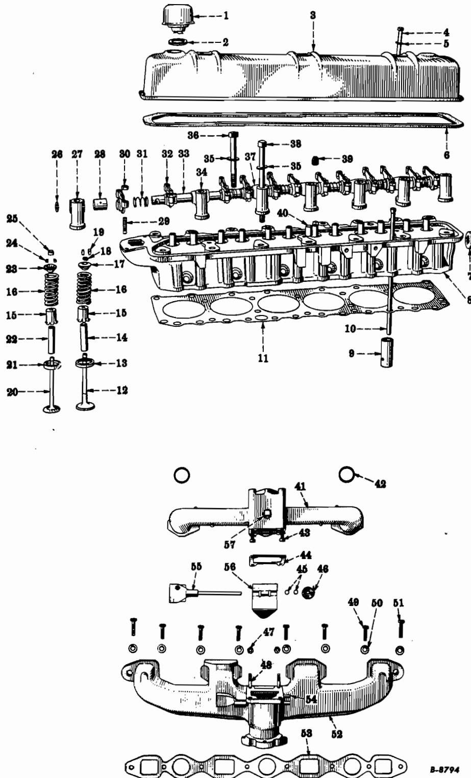
FIG. 12-4 – CYLINDER HEAD AND RELATED PARTS
