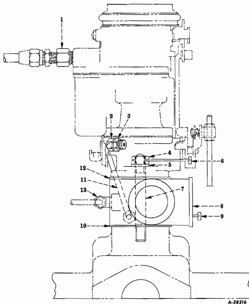
FIG. 12-18 — GOVERNOR AND CARBURETOR MOUNTING (Hoof Governor, Code 1554) (For SD-220 Gasoline Engines, Codes 1201, 1221 And SD-240 Gasoline Engines, Codes 1202, 1212) (R-110 Series - Below 8012) (R-120 Series - 501 To 1452 And 1501 To 1700) (R-130 Series - 501 To 1204 And 2000 To 2083) (R-160 Series - Below 2986) (RC-160 Series - Below 761)
