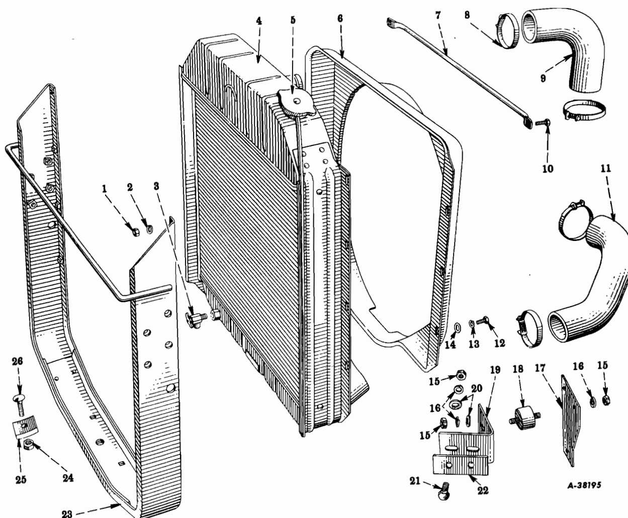
FIG. 12-7 — RADIATOR CORE AND MOUNTING (R-100, R-110, R-120, R-130, R-140-4x4, R-150, R-160, R-160-4x4 Series)
