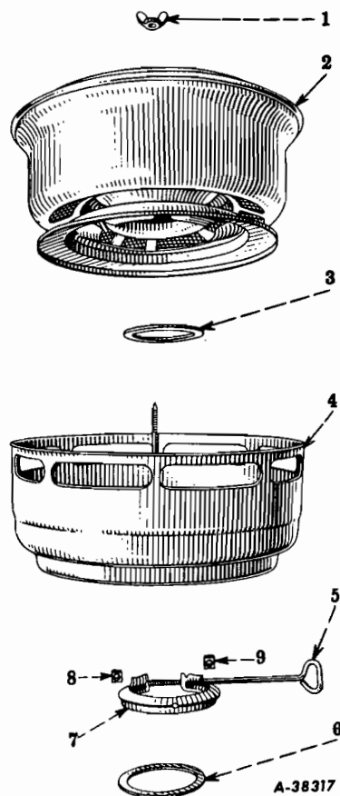
FIG. 12-28 — CARBURETOR AIR CLEANER (Standard) (For SD-220, SD-240 Gasoline Engines With Carter Carburetor) (Not For RC-160 Series)
