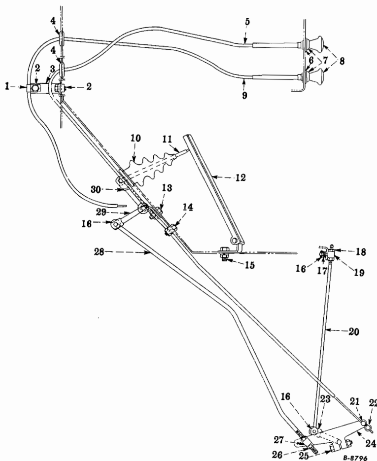
FIG. 12-36 — ACCELERATOR, THROTTLE, AND CHOKE CONTROL (RC-160 Series)
