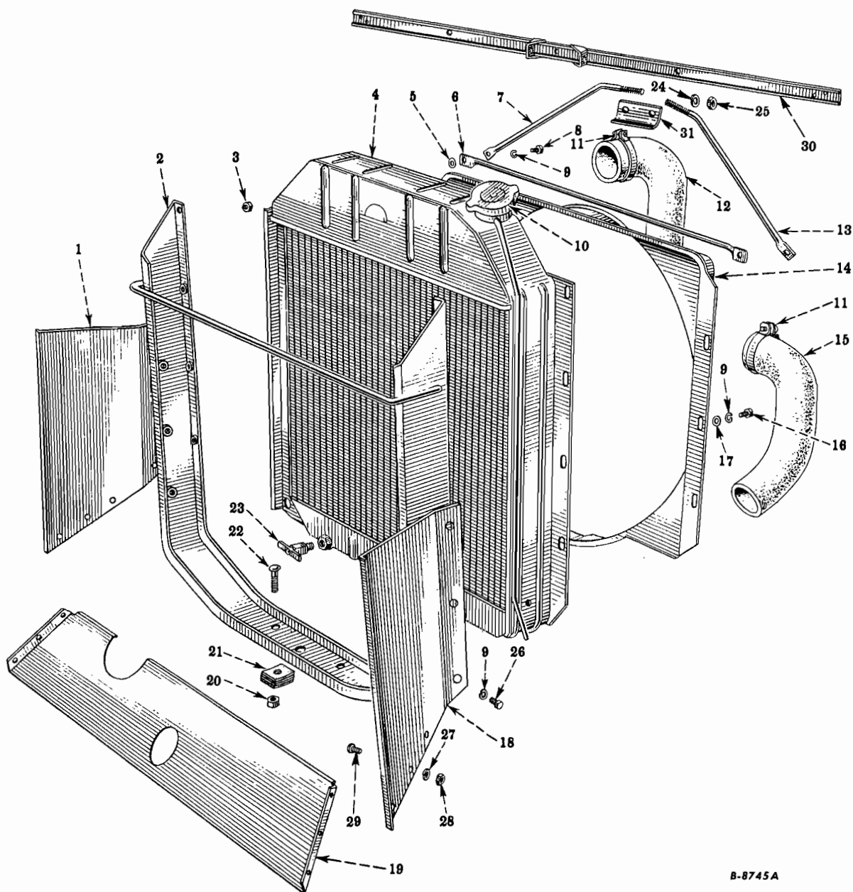
FIG. 12-8 - RADIATOR CORE AND MOUNTING (RC-160 Series)
