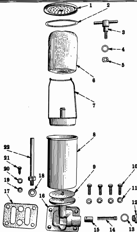
FIG. 12-5 - DELUXE OIL FILTER (Code 1250)
