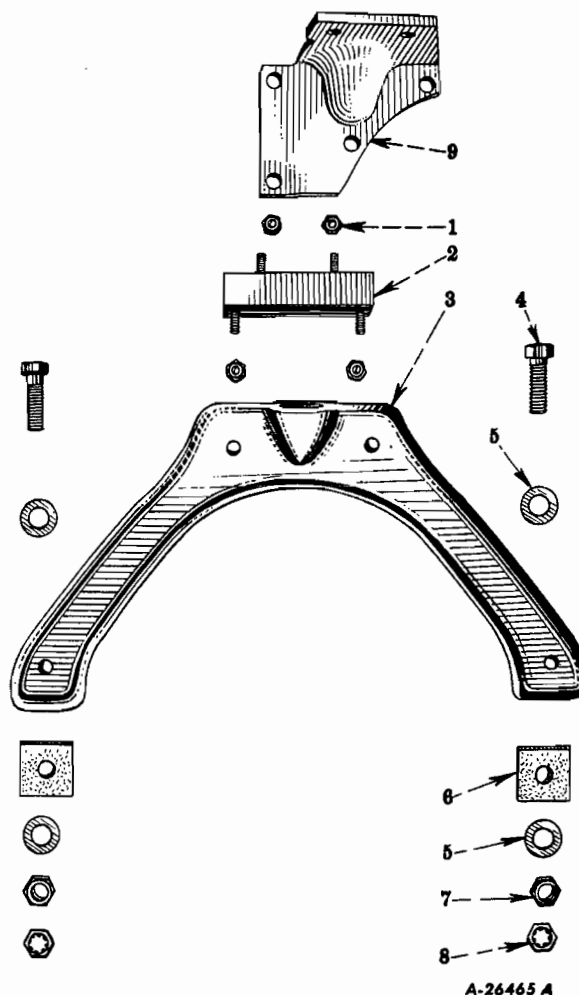
FIG. 12-9 - FRONT MOUNTING
