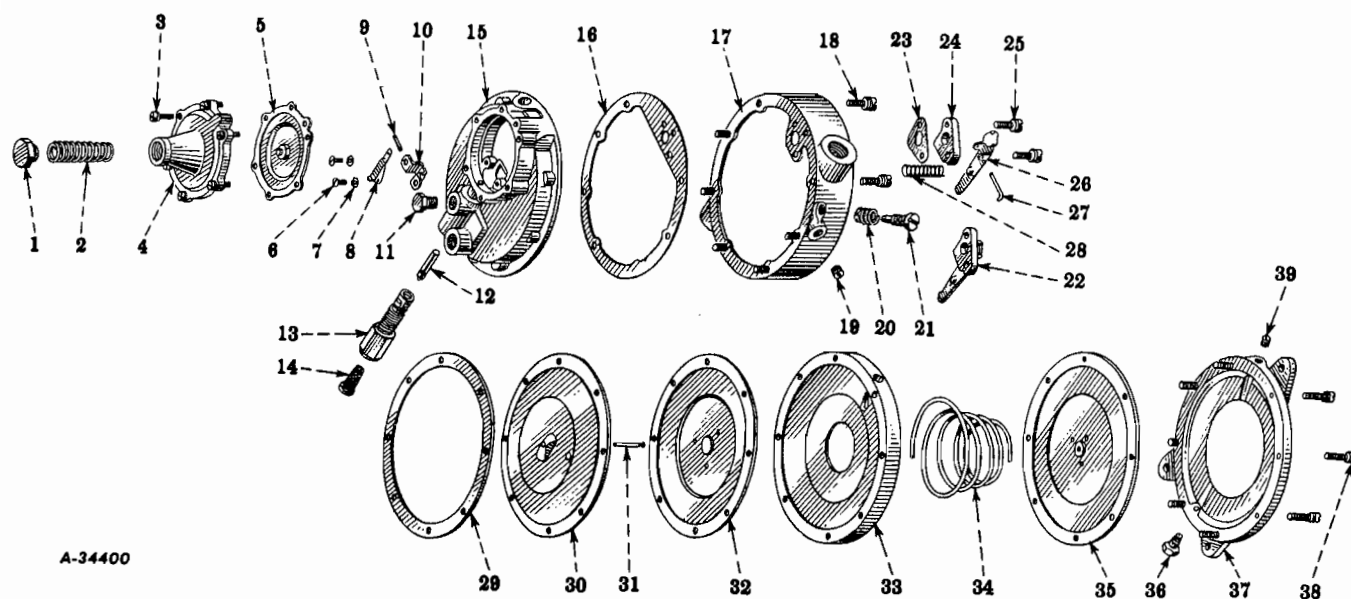
FIG. 12-22 — FUEL REGULATOR (For SD-240, LPG Engines, Code 1231)
