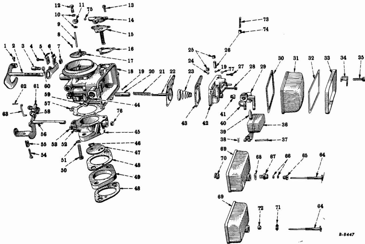
FIG. 12-16 — CARBURETOR (Holley Model 1904) (For SD-220 Gasoline Engines, Codes 1201, 1221 And SD-240 Gasoline Engines, Codes 1202, 1212) (R-100 Series - 501 And Up) (R-110 Series - 8012 And Up) (R-120 Series - 1453 To 1500, Also 1701 And Up) (R-130 Series - 1205 To 1999, Also 2084 And Up) (R-140-4x4 Series - 501 And Up) (R-150 Series - 502 And Up) (R-160 Series - 2986 And Up) (R-160-4x4 Series - 501 And Up) (RC-160 Series - 761 And Up)
