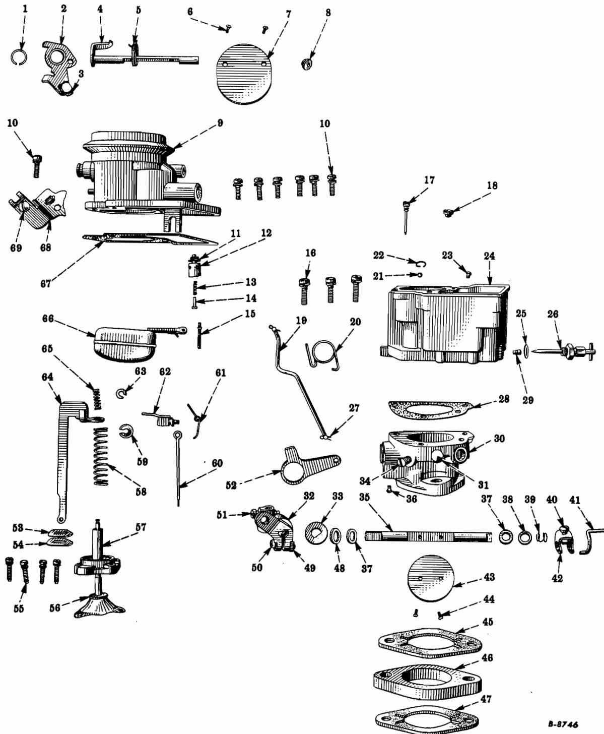
FIG. 12-15 — CARBURETOR (Carter) (For SD-220 Gasoline Engines, Codes 1201, 1221, And SD-240 Gasoline Engines, Codes 1202, 1212) (R-110 Series - Below 8012) (R-120 Series - 501 To 1452 And 1501 To 1700) (R-130 Series - 501 To 1204 And 2000 To 2083) (R-160 Series - Below 2986) (RC-160 Series - Below 761)
