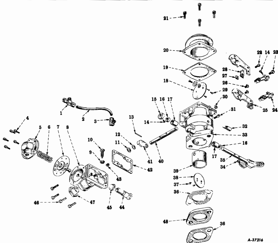
FIG. 12-21 - CARBURETOR (Ensign) (For SD-240 LPG Engines, Code 1231)
