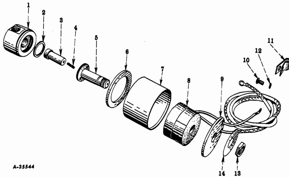
FIG. 12-24 — FUEL SOLENOID VALVE (For SD-240 LPG Engines, Code 1231)
