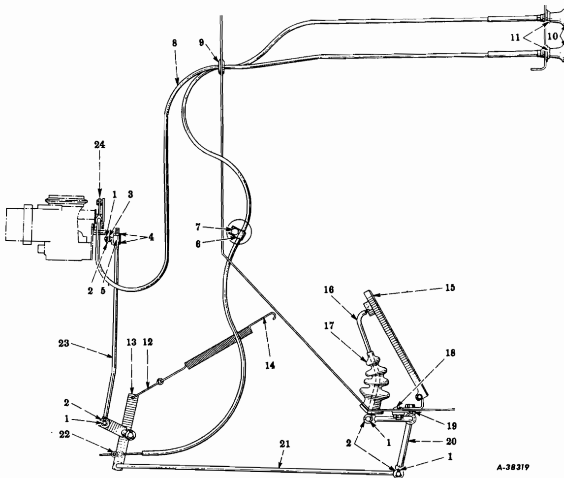
FIG. 12-37 - ACCELERATOR, THROTTLE AND CHOKE CONTROL (Right Hand Drive)
