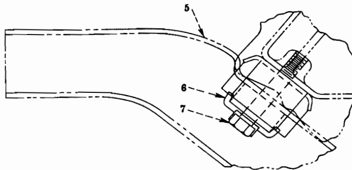
FIG. 12-11 — REAR MOUNTING (R-100, R-110, R-120, R-130 Series With Transmission Code 1374)
