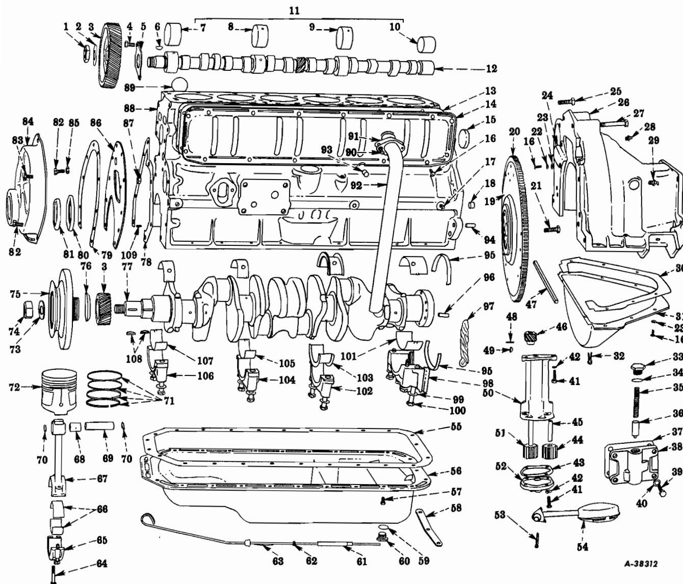
FIG. 12-2 — CRANKCASE AND RELATED PARTS
