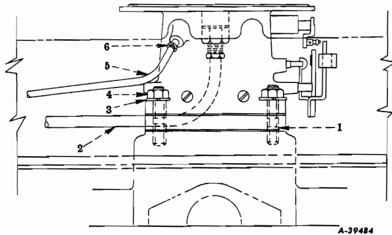
FIG. 12-14A - CARBURETOR MOUNTING (For BD-264 Engines, Code 1222)
