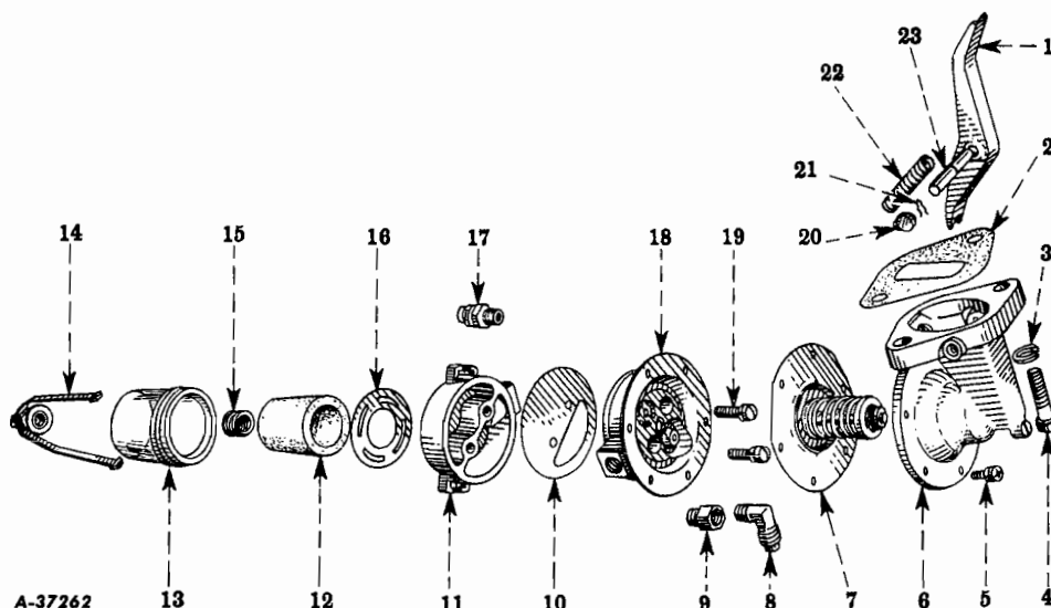
FIG. 12-26 - FUEL PUMP (Carter) (For Gasoline Engines)
