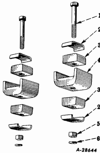
FIG. 12-10 — REAR MOUNTING (R-100, R-110, R-120, R-130 Series - With SD-220 Engine, Except With Transmission Code 1374)
