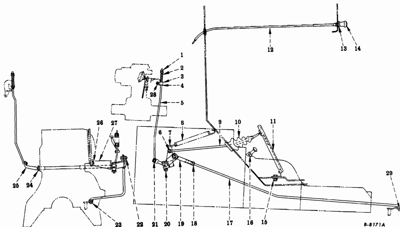
FIG. 12-35 - ACCELERATOR, THROTTLE AND CHOKE CONTROL (For Transmission Code 1374)
