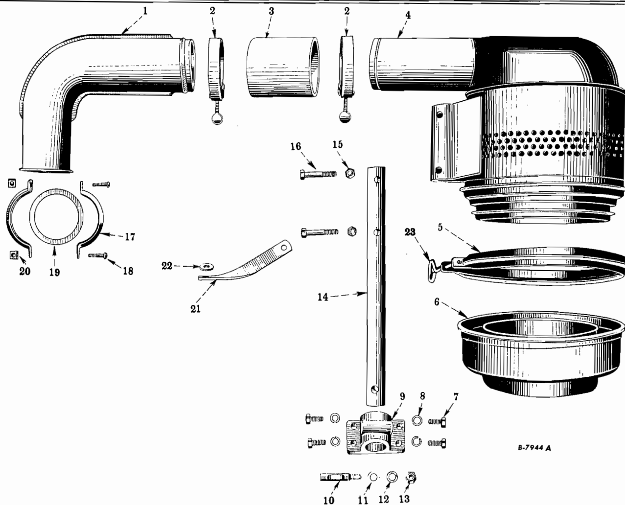
FIG. 12-32 – CARBURETOR AIR CLEANER (Heavy Duty, Code 1552) (For SD-220, SD-240 Engines) (All Series Except RC-160)
