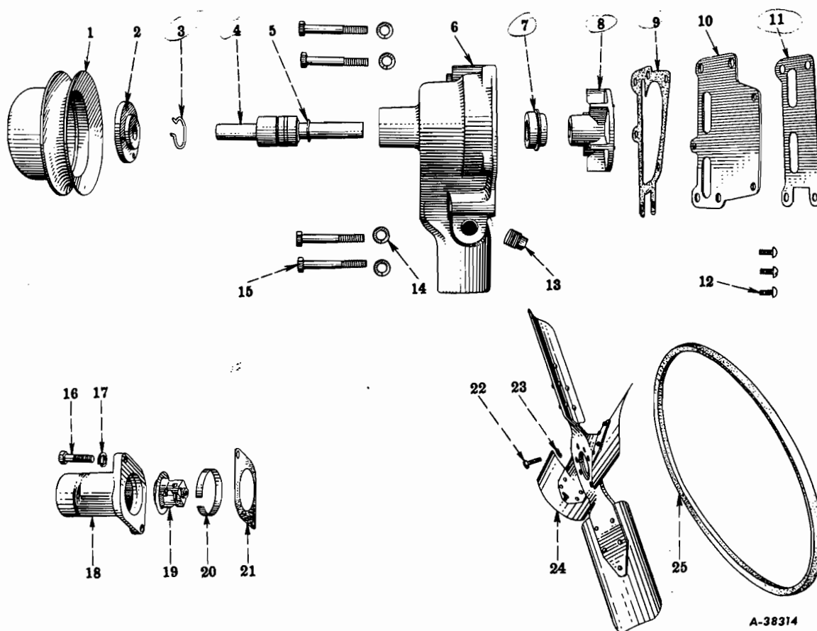
FIG. 12-6 – WATER OUTLET, THERMOSTAT, WATER PUMP, FAN AND FAN BELT
