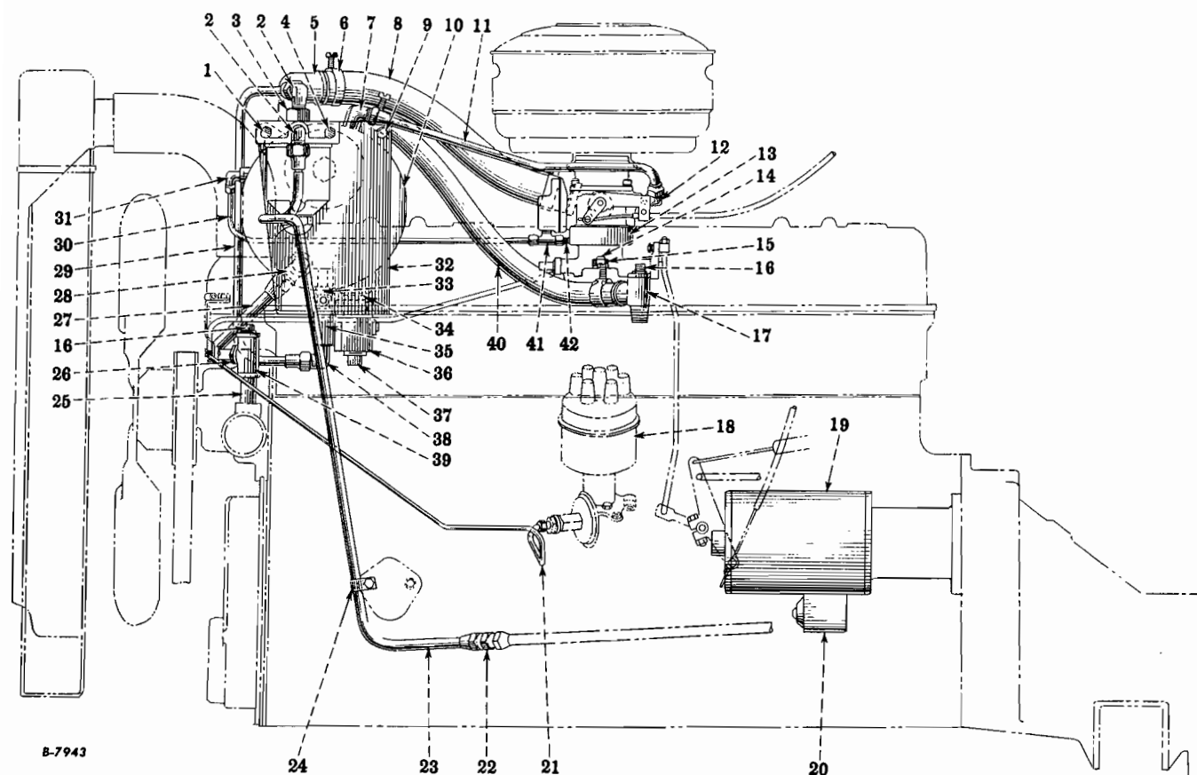
FIG. 12-20 — LPG ENGINE EQUIPMENT AND MOUNTING (SD-240 LPG Engine, Code 1231)
