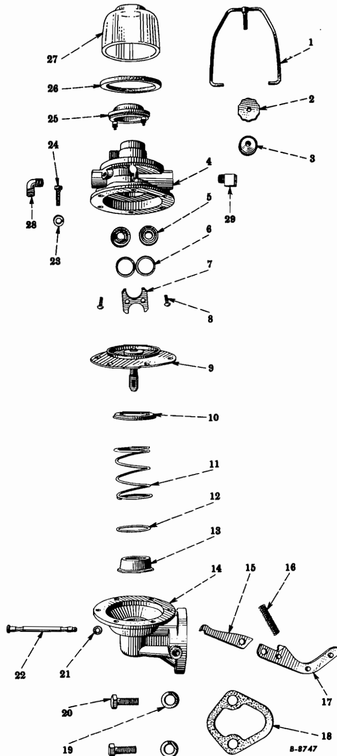
FIG. 12-27 — FUEL PUMP (AC) (For Gasoline Engines)
